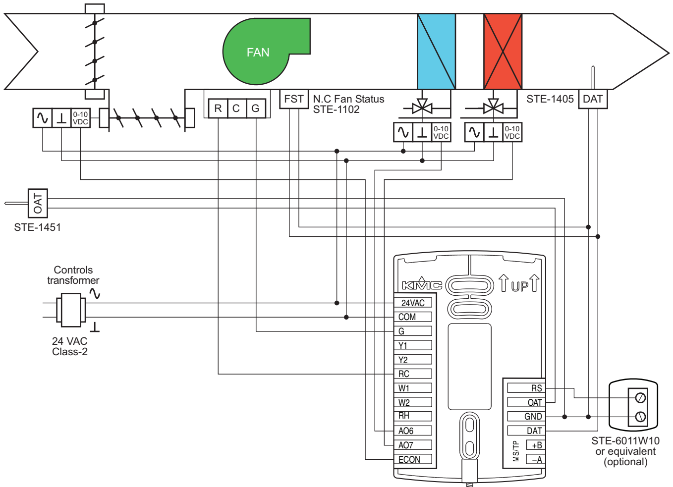
Illustration 6-12 Wiring details: RTU with modulating valves cooling and heating valves and economizer
