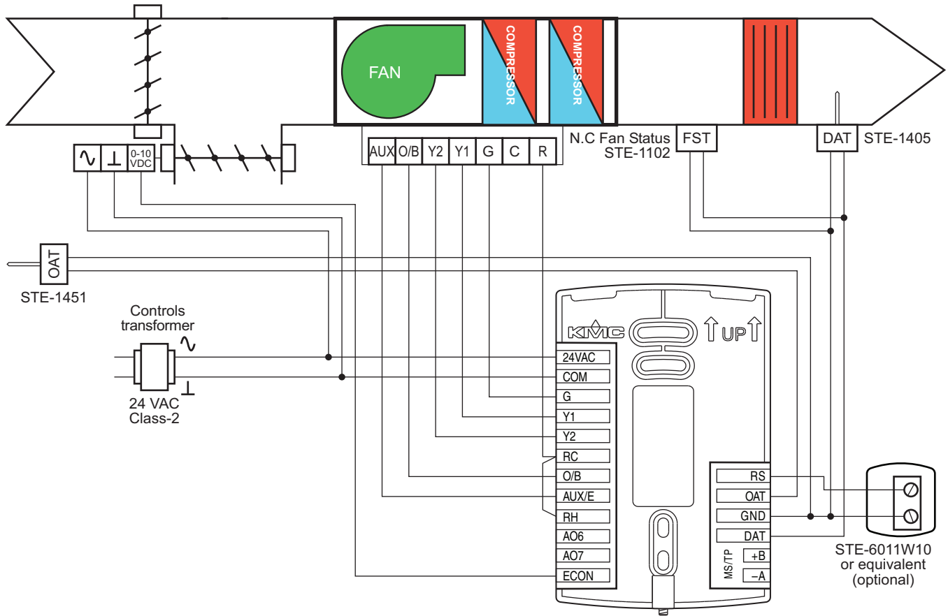
Illustration 6-14 Wiring details: HPU with three heat, two cool and economizer
