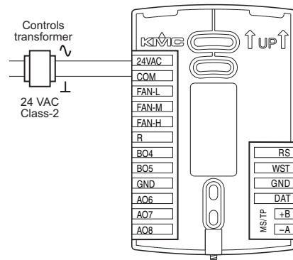
Illustration 2–12 Wiring for AppStat power
