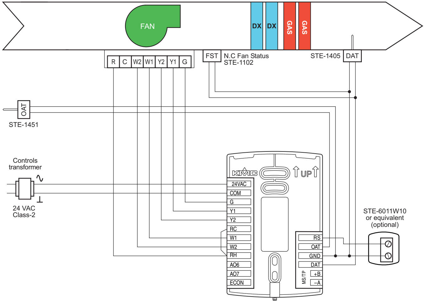
Illustration 6-9 Wiring details: RTU two-stage gas heat and two-stage DX cooling
