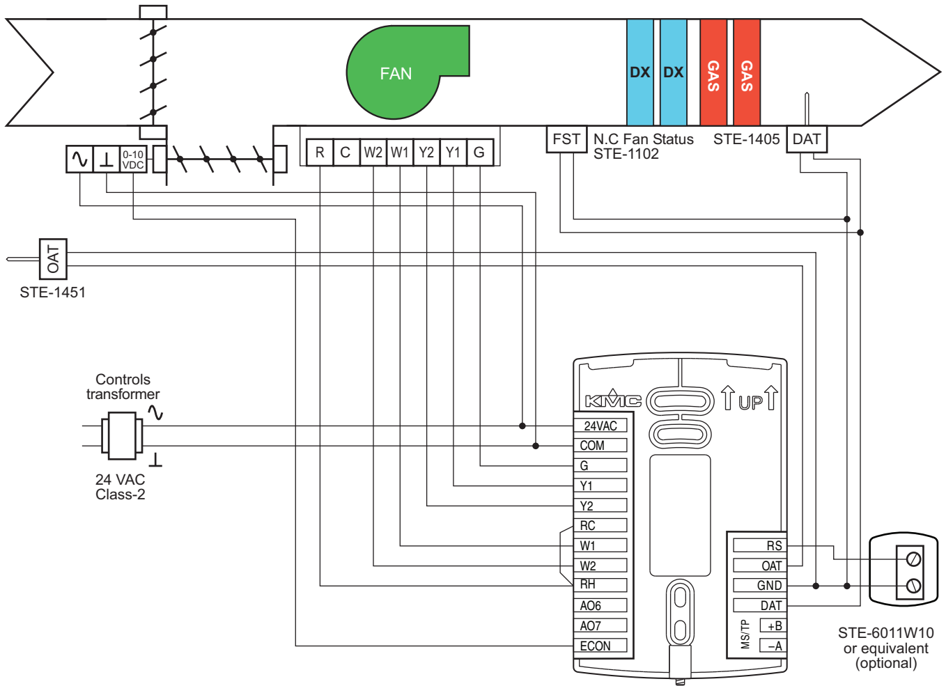
Illustration 6-10 Wiring details: RTU two-stage gas heat and two-stage DX cooling and economizer
