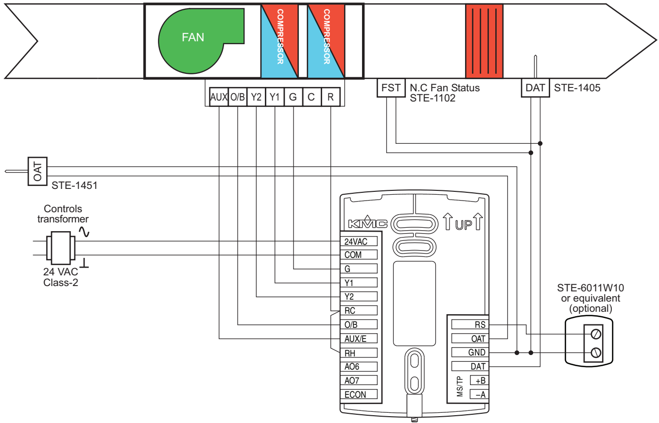
Illustration 6-13 Wiring details: HPU—Three heat, two cool
