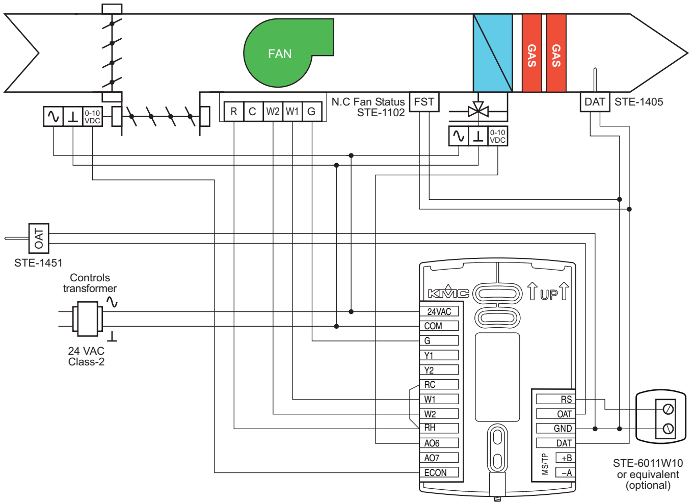
Illustration 6-11 Wiring details: RTU with two-stage gas heat, chilled water cooling with economizer
